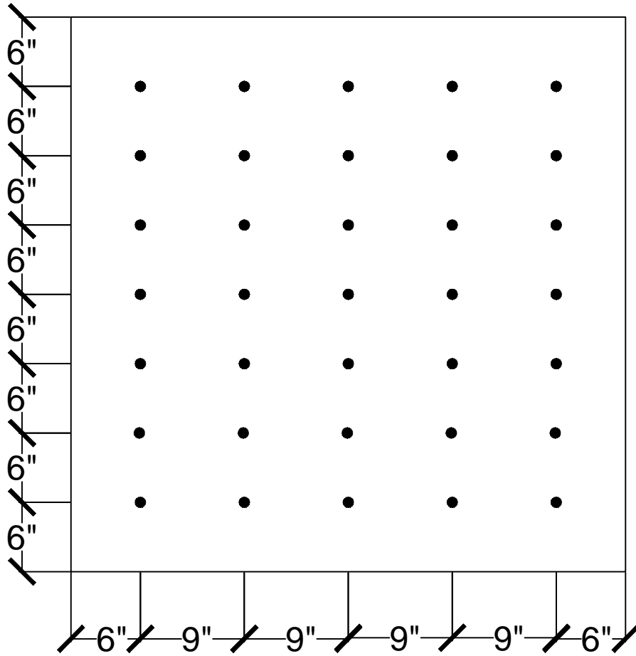
35 FASTENERS PER 4' x 4' BOARD
