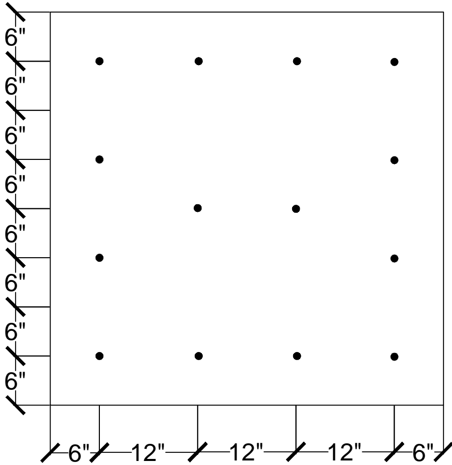
14 FASTENERS PER 4' x 4' BOARD
